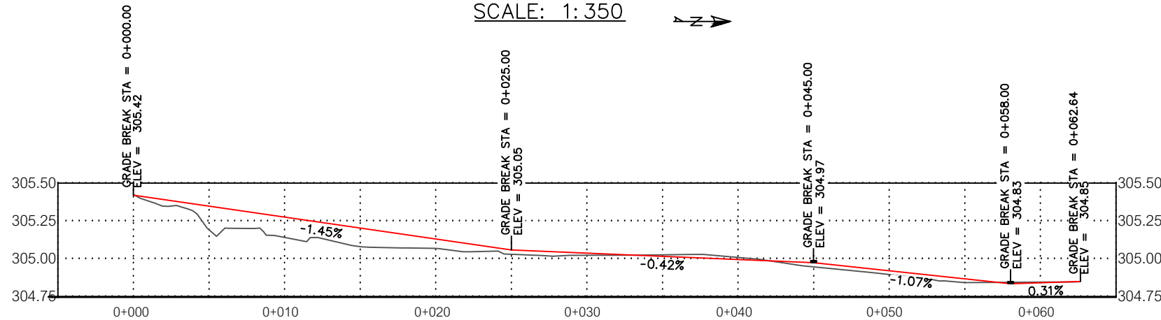
13TH ST REPAIR PROFILE SCALE: 1:350
