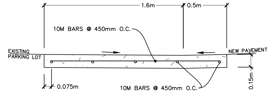
REINFORCED CONCRETE DETAIL SCALE: 1:25
