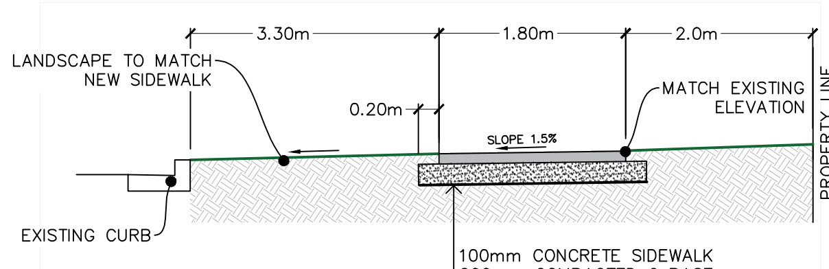
1 CROSS SECTION SCALE 1:50
