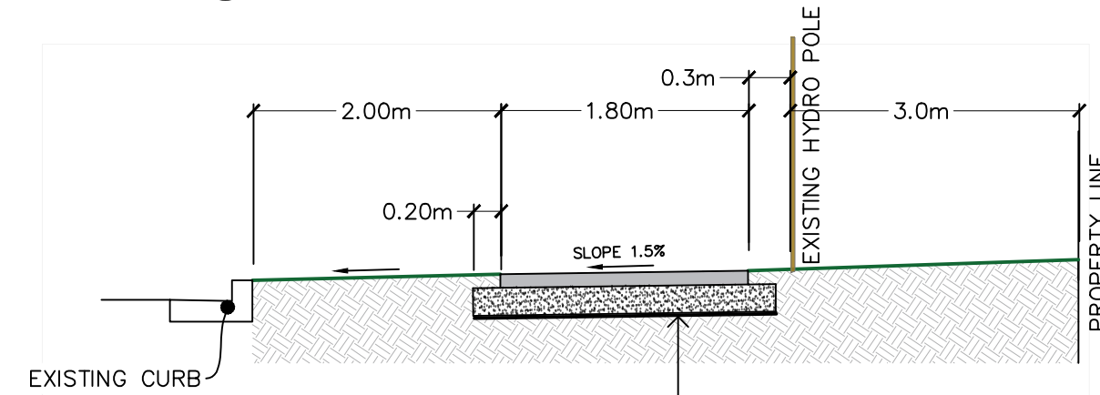
1 CROSS SECTION SCALE 1:50
